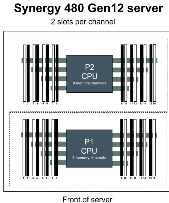
Figure 6. DIMM slot locations for 480 Gen12 servers with 6th Gen Intel Xeon compute modules (P1 and P2 are rotated.)
